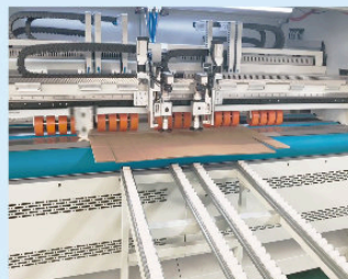
Vibrating Knife Cutting (Option)
